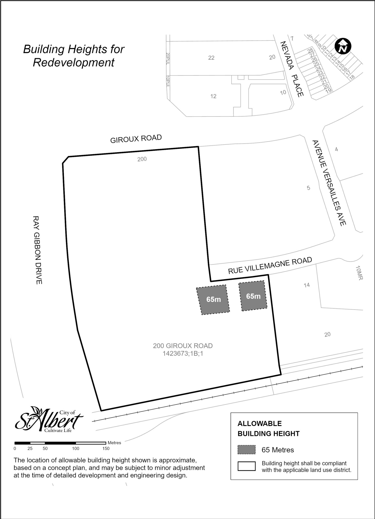
Figure 11-3: Building Heights for Redevelopment, Ville Giroux Neighbourhood
